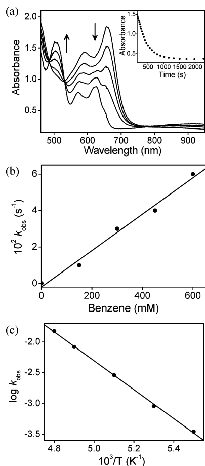
FIGURE 1. (a) UV-vis spectral changes of 1 (1.5 mM) upon addition of 100 equiv of benzene in \text{CH}_2\text{Cl}_2 at -80\text{ }^\circ\text{C} . Inset shows absorbance traces monitored at 660 nm. (b) Plot of k_{\text{obs}} against benzene concentration to determine a second-order rate constant at -80\text{ }^\circ\text{C} . (c) Plot of first-order-rate constants against 1/T to determine activation parameters.
